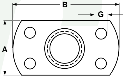
TAB WELD NUTS - CENTER HOLE DESIGN WITH MULTIPLE PROJECTIONS
