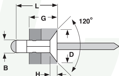
COUNTERSUNK
