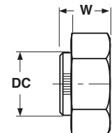
Hex Collar-type
